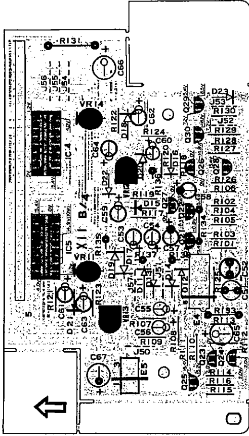
PC BOARD (X11-1670-10) Component side view
