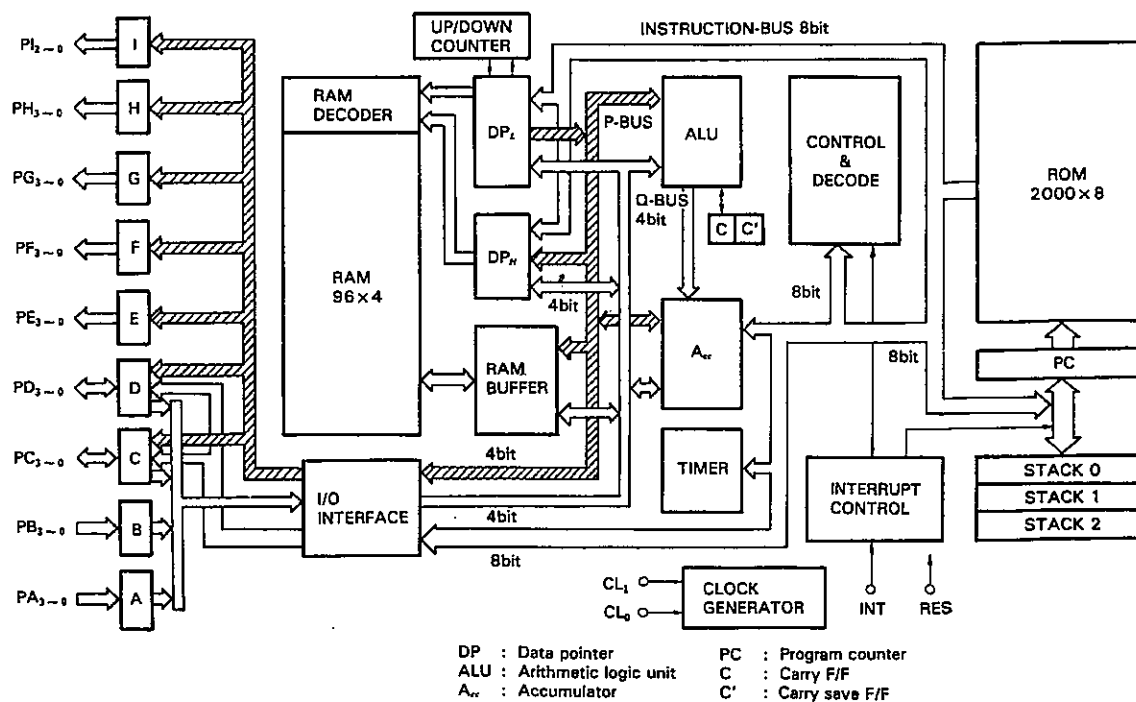
Fig. 14 Block Diagram
