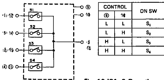
Fig. 10 IC1, 3 Operation
