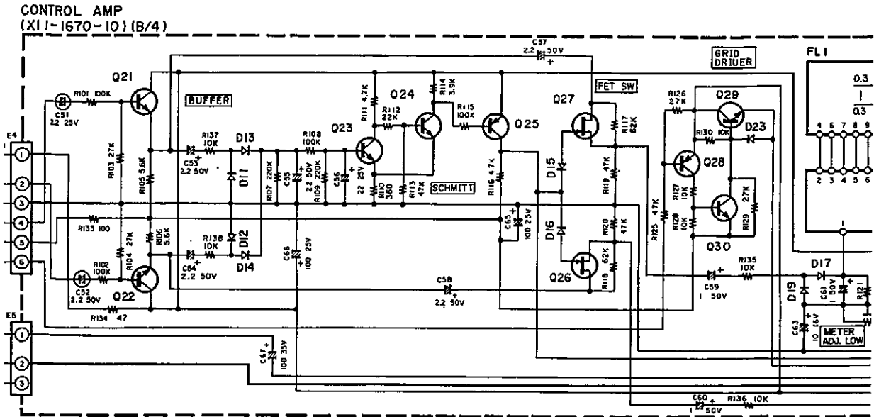
Fig. 20 Automatic Power Meter Range Switching Circuit
